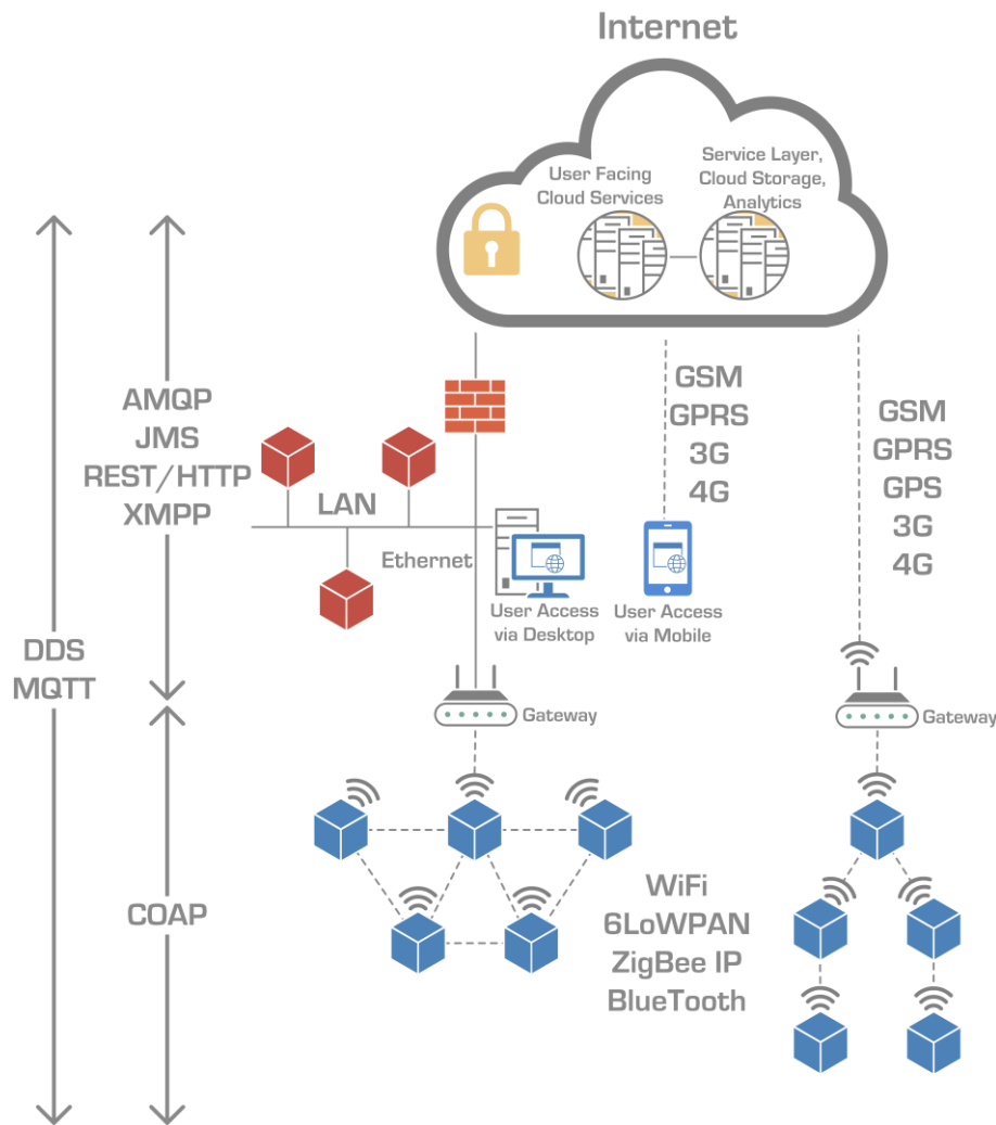
Figure 1 – IoT Connectivity Problem Space
